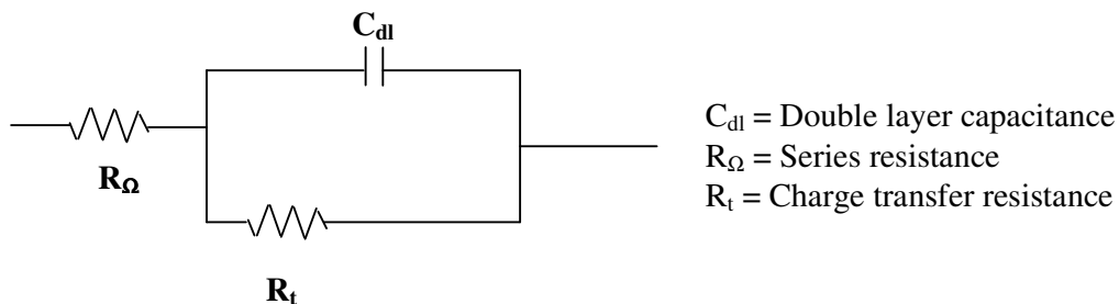
Scheme 2. Modified equivalent circuit of electrode impedance
