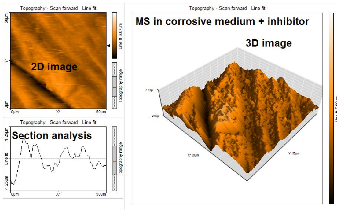
Figure 18. 2D, 3D images and section analysis for inhibited metal.
