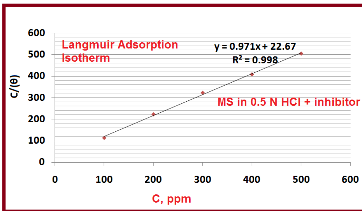
Figure 6. Langmuir adsorption isotherm.
