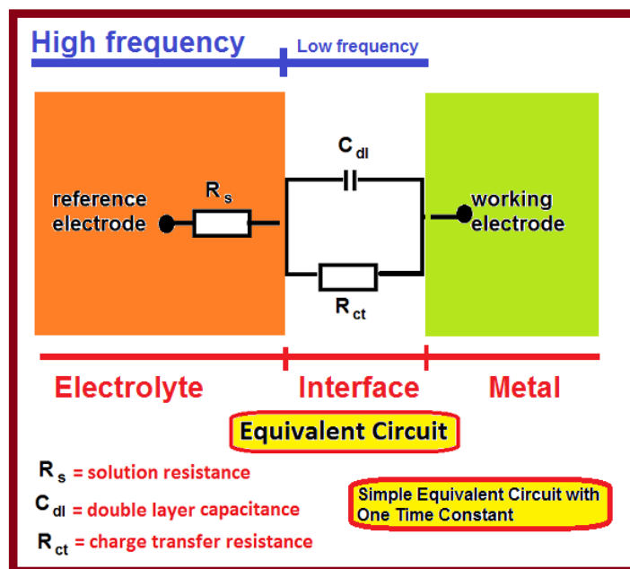
Figure 11. Equivalent circuit with one time constant.
